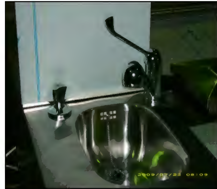
Sink with 25mm radius, elbow operated taps with flexible hose 1500mm long. Left: Valve for operation of sprinkler system below work area
